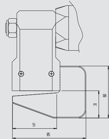
TA12 Tool head
